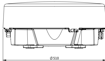
LEFT VIEW
